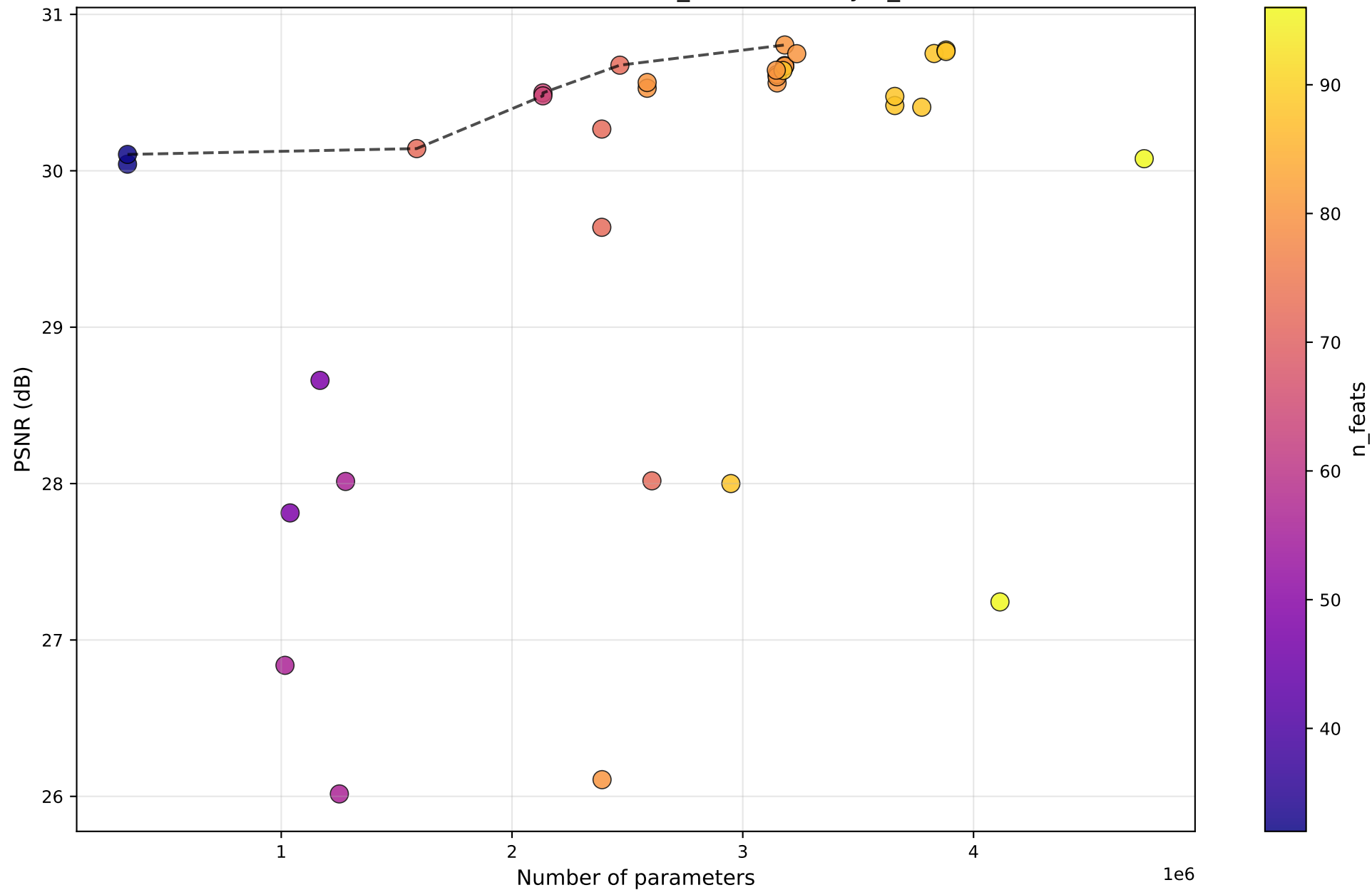
PSNR vs #Params — DHTCUN_baseline — by n_feats
